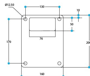
Floor Bracket Hole Positions
